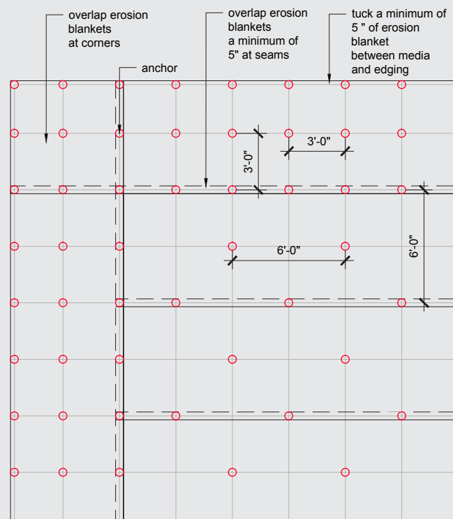
Typical Blanket and Anchor Layout
